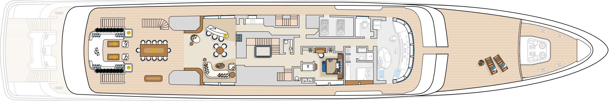
BRIDGE DECK
