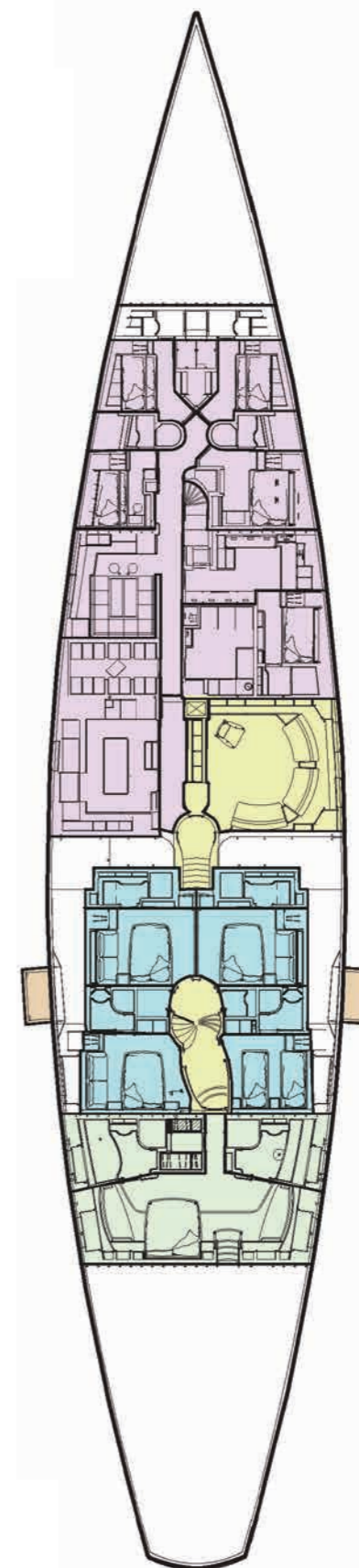
LOWER DECK
