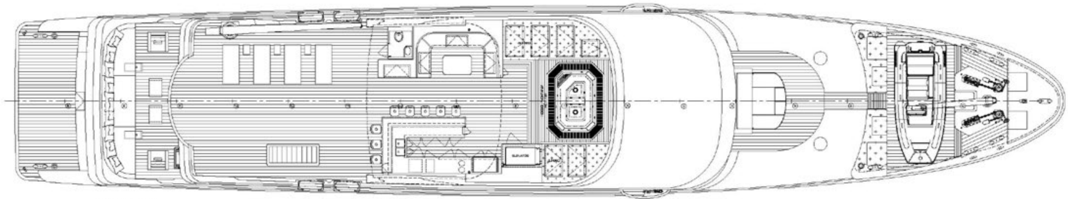
SUNDECK PLAN
