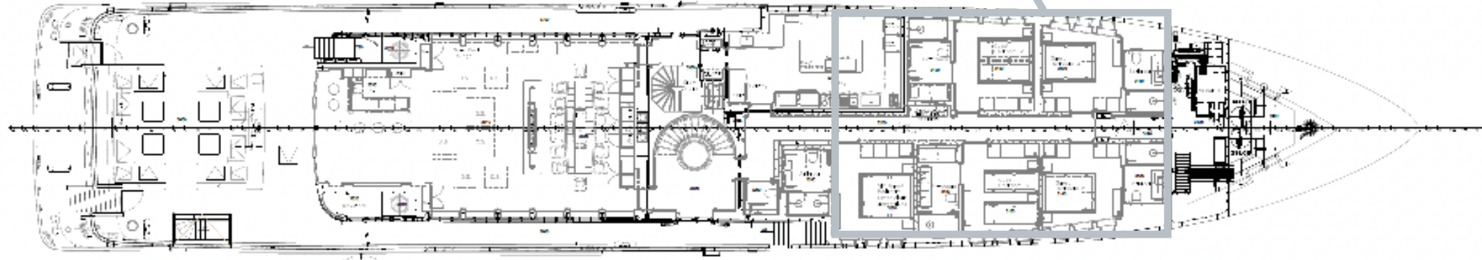
MAIN DECK ACCOMMODATIONS
