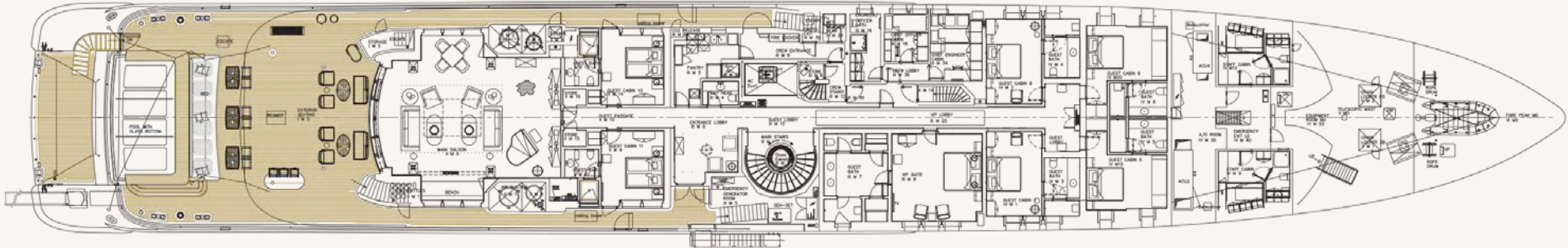
MAIN DECK
