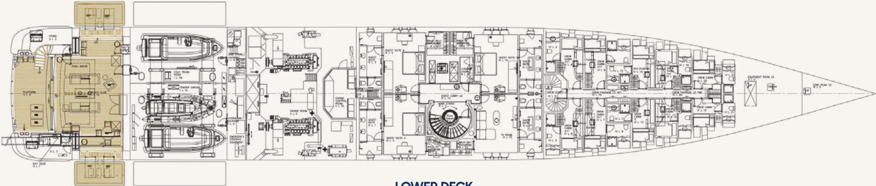
LOWER DECK
