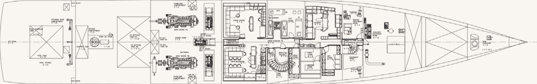
TANK DECK
