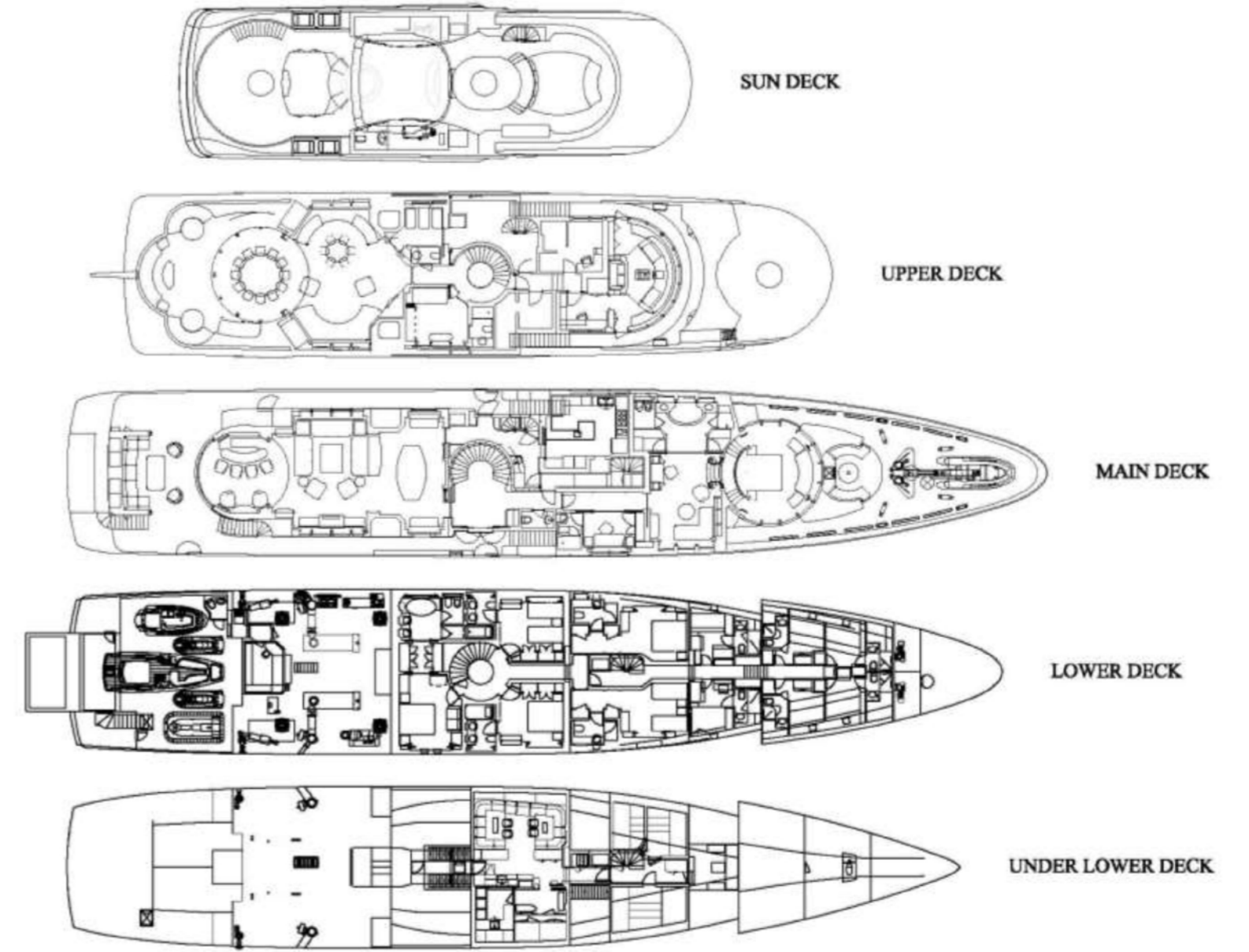
St. David Deck Plan
